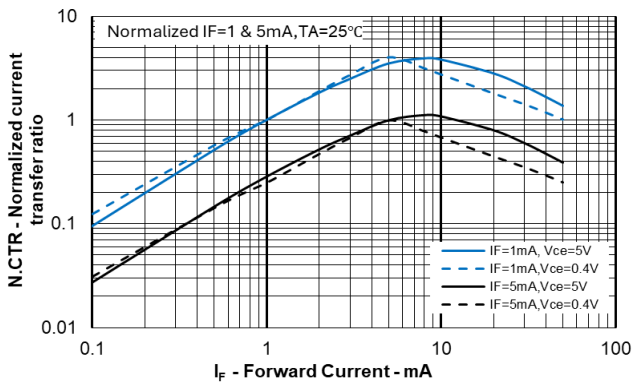
Fig.5 Normalized current transfer ratio vs Forward current.
