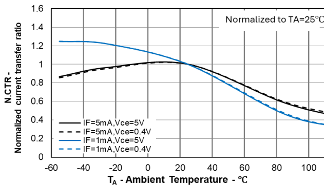
Fig.7 Normalized current transfer ratio vs Ambient Temperature.
